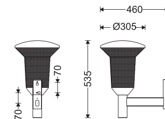
WT3-Bracket
