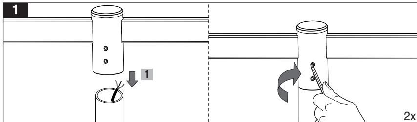
PTT2-Bracket
