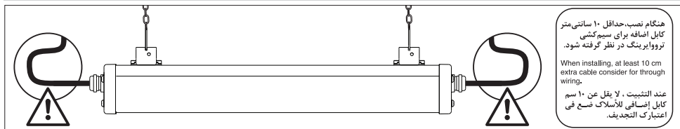
Through wiring
