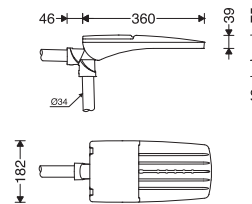
M320SULED1... M320SULED2...
