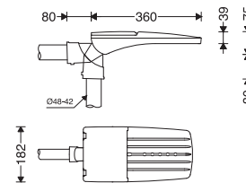
M320SULED3... M320SULED4...
