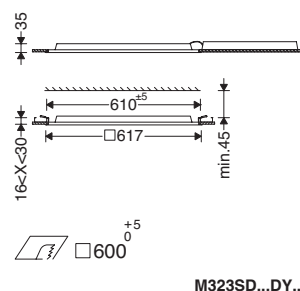
M323SD...DY...
