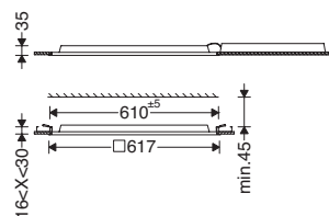
M323SDLED...
