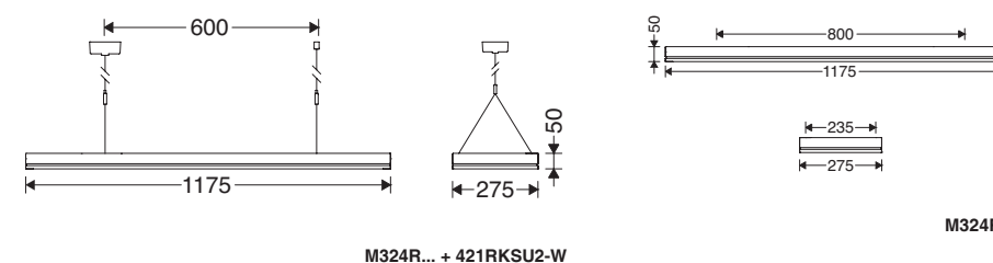
M324R... + 421RKSU2-W
